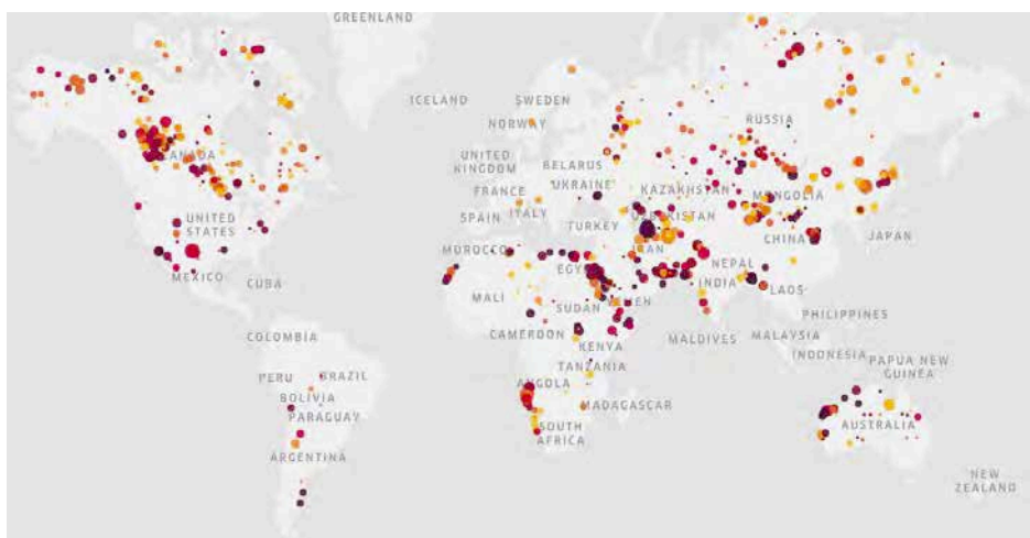
Figure 4. This image shows a sample of abnormal methane concentrations over 2019 as measured by Sentinel-5P. The size and colour of the circles indicate the size and intensity of the plume detected. The redder the colour, the higher the concentration of the methane plume. This image contains modified Copernicus Sentinel data (2019), processed by Kayros.
