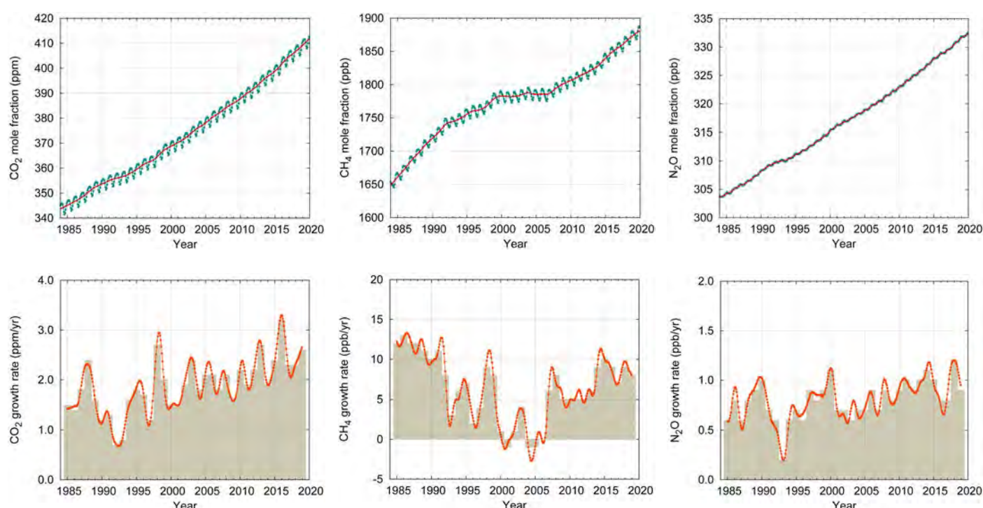
Figure 1. (upper row) Globally averaged \text{CO}_2 , \text{CH}_4 and \text{N}_2\text{O} mole fraction in ppm ( \text{CO}_2 ) and ppb ( \text{CH}_4 ; \text{N}_2\text{O} , respectively) and its growth rates (bottom row) from 1984 to 2019. Increases in successive annual means are shown as the shaded columns in the bottom row. The red line in the upper row is the monthly mean with the seasonal variation removed; the blue dots and line depict the monthly averages
