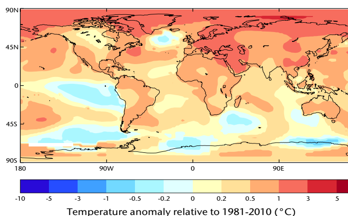
Figure 2. 2017–2021 five-year average temperature anomalies relative to the 1981–2010 average. Data is from NASA GISTEMP v4. Date updated to July 2021
