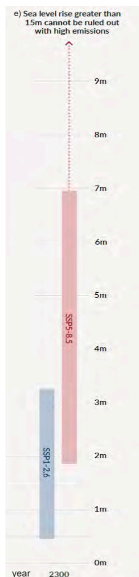
Figure 1. Panels d) and e) from Figure SPM.8 in IPCC AR6 Working Group 1 Summary for Policy Makers (IPCC, 2021). Panel d) Global mean sea level change in meters relative to 1900. The historical changes are observed (from tide gauges before 1992 and altimeters afterwards), and the future changes are assessed consistently with observational constraints based on emulation of CMIP, ice sheet, and glacier models. Likely ranges are shown for SSP1-2.6 and SSP3-7.0. Only likely ranges are assessed for sea level changes due to difficulties in estimating the distribution of deeply uncertain processes. The dashed curve indicates the potential impact of these deeply uncertain processes. It shows the 83rd percentile of SSP5-8.5 projections that include low-likelihood, high-impact ice sheet processes that cannot be ruled out; because of low confidence in projections of these processes, this curve does not constitute part of a likely range. Changes relative to 1900 are calculated by adding 0.158 m (observed global mean sea level rise from 1900 to 1995–2014) to simulated and observed changes relative to 1995–2014. Projected sea-level rise 1900 to 2100 for a range of emission scenarios. Panel e): Global mean sea level change at 2300 in meters relative to 1900. Only SSP1-2.6 and SSP5-8.5 are projected at 2300, as simulations that extend beyond 2100 for the other scenarios are too few for robust results. The 17th–83rd percentile ranges are shaded. The dashed arrow illustrates the 83rd percentile of SSP5-8.5 projections that include low-likelihood, high-impact ice sheet processes that cannot be ruled out.
